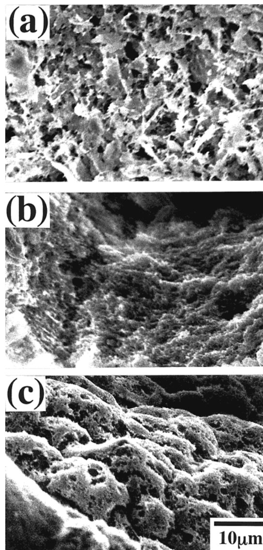
Figure 8. Scanning electron micrographs of porous ceramic materials obtained after burning the nanocomposites with C 16 modifier and same clay content (5 wt %): (a) PLACN10 (mica), (b) PLACN7 (MMT), and (c) PLACN4 (smectite).
