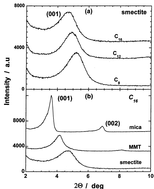
Figure 2. WAXD patterns of organically modified clay: (a) smectite clay modified with \text{C}_8 , \text{C}_{12} , and \text{C}_{16} phosphonium salt; (b) smectite, MMT, and mica clay modified with \text{C}_{16} phosphonium salt.
