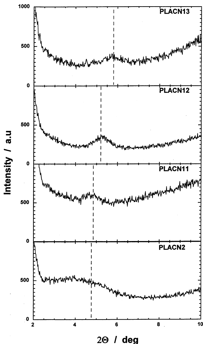
Figure 3. WAXD patterns of smectite-organoclay nanocomposites having different organic components (chain length dependency on intercalation). The broken lines represent the peak position of the corresponding organoclay.
